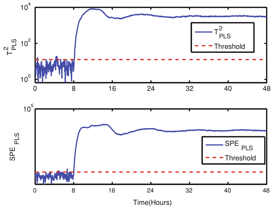
Fig. 6.3 PLS based fault detection results for fault scenario 1
