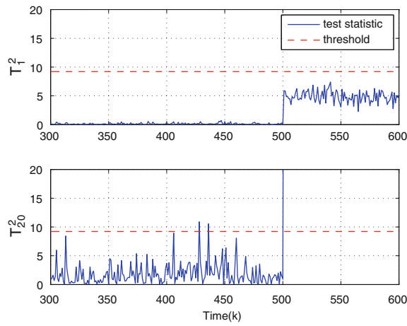
Fig. 12.19 T^2 test statistics at the 1st and 20th iterations
