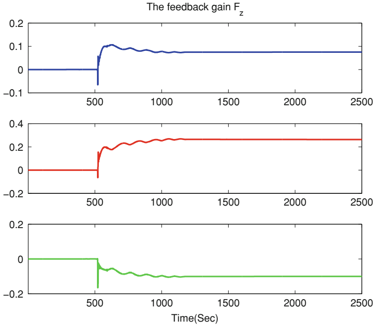
Fig. 15.6 Update of F_z
