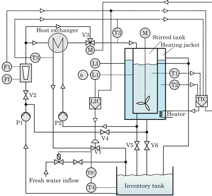
Fig. 2.2 Laboratory setup CSTD
