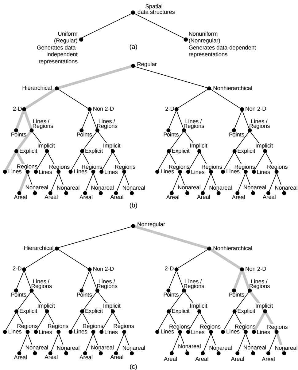
FIGURE 18.8 Spatial data structure taxonomies with the recommended representation branches outlined in bold gray lines.
