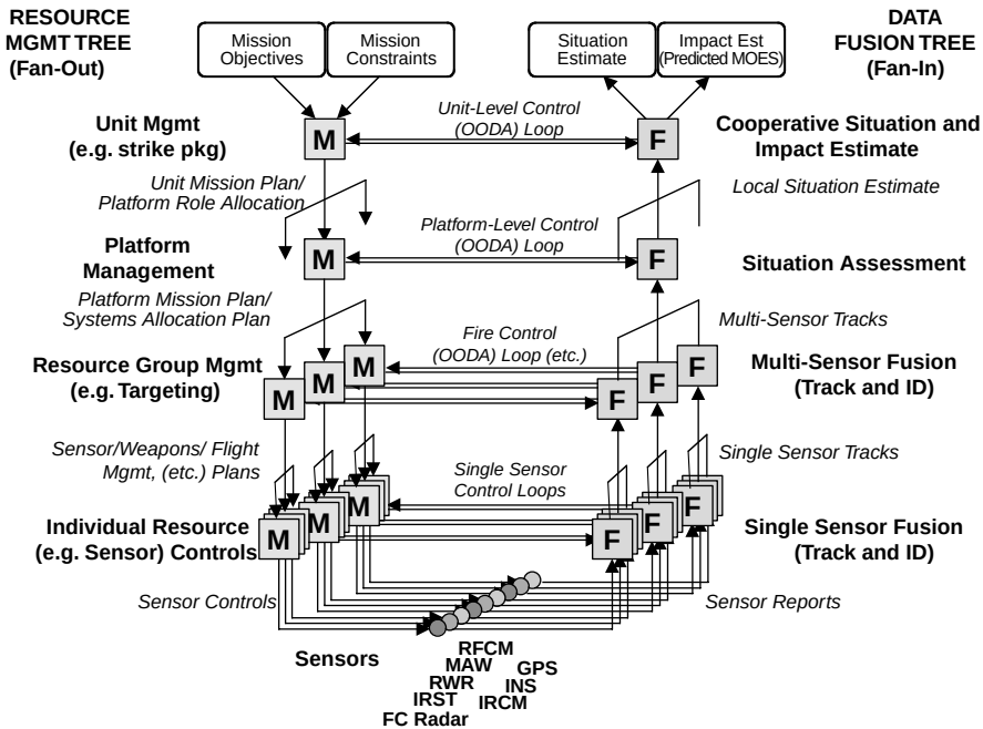
FIGURE 16.12 Dual DF/RM tree architecture for fighter aircraft.
