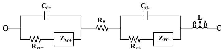
FIGURE 23.25 Two-electrode Randles circuit model with wiring inductance.
