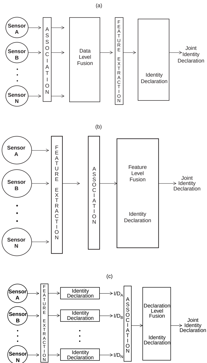
FIGURE 1.4 (a) Direct fusion of sensor data. (b) Representation of sensor data via feature vectors and subsequent fusion of the feature vectors. (c) Processing of each sensor to achieve high-level inferences or decisions that are subsequently combined.
