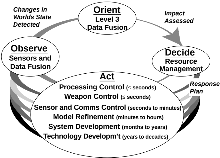
FIGURE 16.16 Resource management at multiple levels of granularity.
