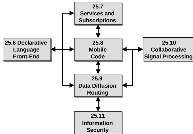
FIGURE 25.3 Functional decomposition of the SenseIT software architecture. Numbers refer to chapter sections describing the functionality.
