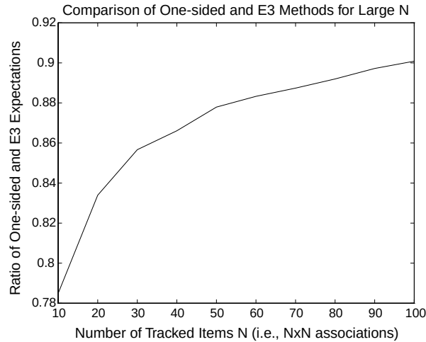
FIGURE 9.4 The performance of the one-sided approach relative to \epsilon_3 improves with increasing N . This is somewhat misleading, however, because the expected number of correct assignments goes to zero in the limit N \rightarrow \infty for both approaches.
