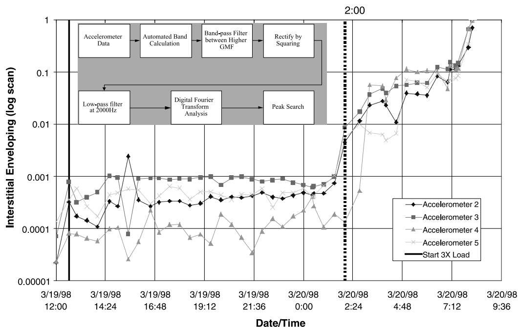
FIGURE 23.11 Interstitial enveloping of accelerometer.
