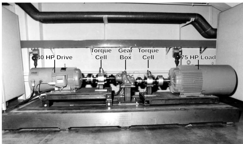
FIGURE 1.3 Mechanical diagnostic testbed used by The Pennsylvania State University to perform condition-based maintenance research.
